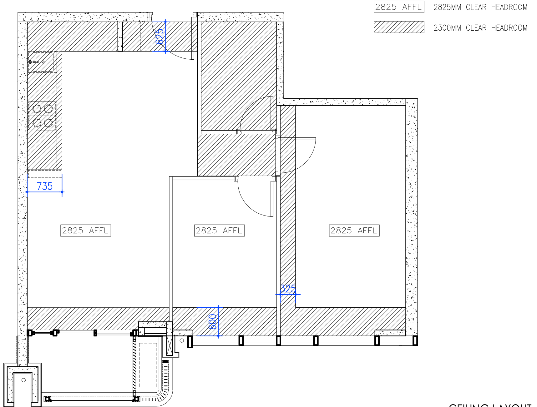
CEILING LAYOUT
